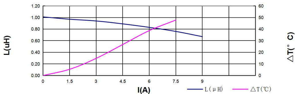
CURRENT CHARACTERISTIC
