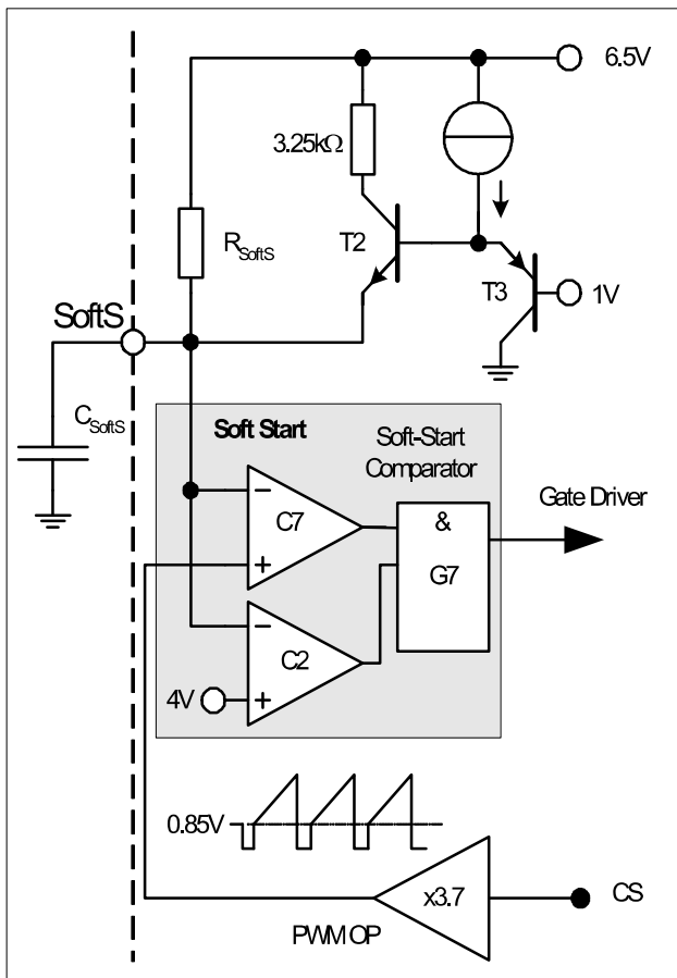
Figure 7 Soft Start
