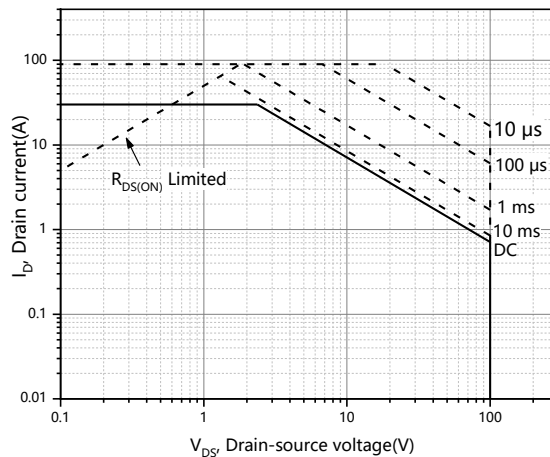
Figure 10. Safe operation area T_C = 25^\circ\text{C}
