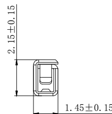
SECTION C-C
