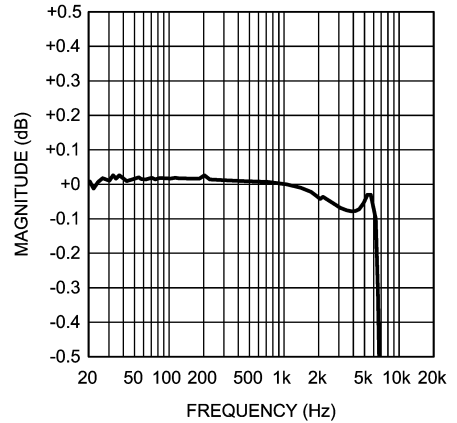
MONO ADC Frequency Response Zoom f_s = 16\text{kHz} , 36dB MIC
