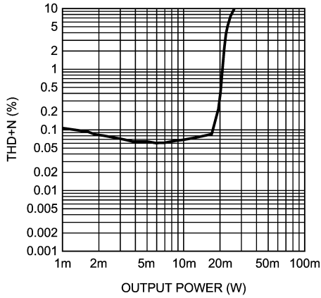
Headphone THD+N vs Output Power AV_{DD} = 5V , OCL 1.2V, 12dB DAC f_{OUT} = 1kHz , 32Ω
