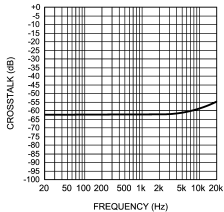
Headphone Crosstalk vs Frequency
