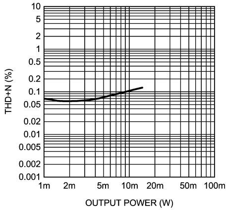
Headphone THD+N vs Output Power AV_{DD} = 5V , OCL 1.5V, 0dB DAC f_{OUT} = 1kHz , 16Ω
