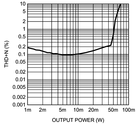
Headphone THD+N vs Output Power AV_{DD} = 3.3V , OCL 1.5V, 12dB DAC f_{OUT} = 1kHz , 16Ω
