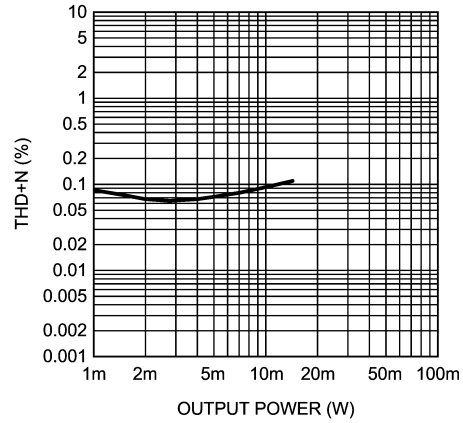
Headphone THD+N vs Output Power AV_{DD} = 3.3V , OCL 1.5V, 0dB DAC f_{OUT} = 1kHz , 16Ω
