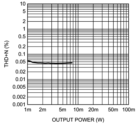
Headphone THD+N vs Output Power AV_{DD} = 3.3V , OCL 1.5V, 0dB DAC f_{OUT} = 1kHz , 32Ω
