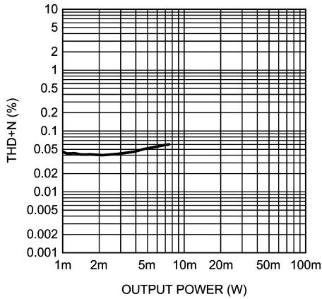
Headphone THD+N vs Output Power AV_{DD} = 5V , OCL 1.5V, 0dB DAC f_{OUT} = 1kHz , 32Ω
