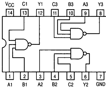
LOGIC DIAGRAM
