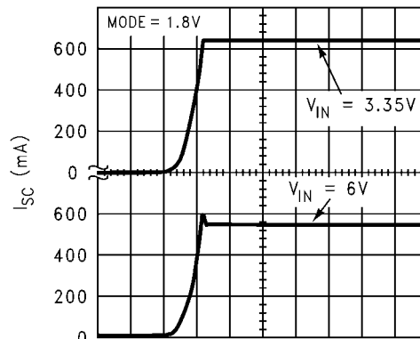
TIME (500 μs/DIV)
