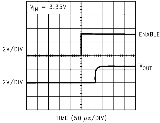
T ON @ MODE = 1.8V, C OUT = 1μF, I L = 150mA
