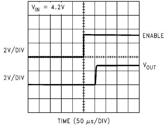
T ON @ MODE = 1.8V, C OUT = 1μF, I L = 150mA
