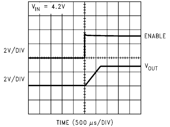
T SLEEP @ MODE = 0V, C OUT = 4.7μF, I L = 1mA
