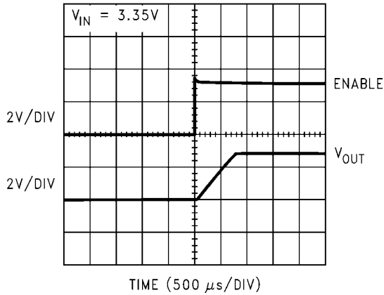
T SLEEP @ MODE = 0V, C OUT = 4.7μF, I L = 1mA
