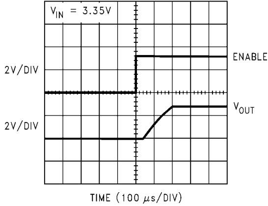
T SLEEP @ MODE = 0V, C OUT = 1μF, I L = 1mA
