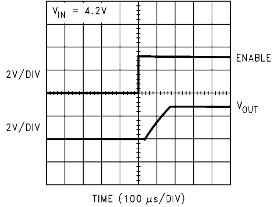
T SLEEP @ MODE = 0V, C OUT = 1μF, I L = 1mA
