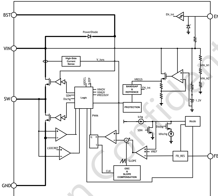
Fig.22 PL88103 Diagram
