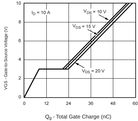
Fig 8. Gate Charge
