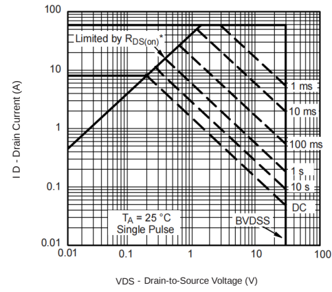
Fig 10. Safe Operating Area
