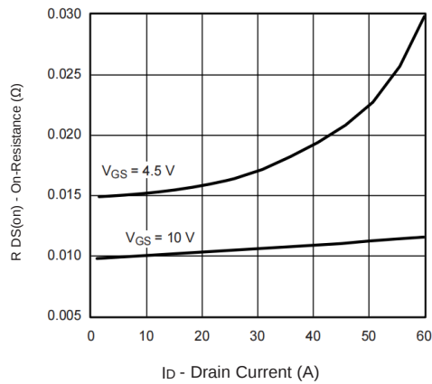
Fig 9. On-Resistance vs. Drain Current
