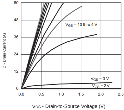
Fig 7. Output Characteristics
