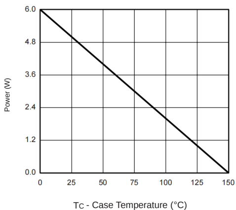
Fig 11. Power, Junction-to-Foot
