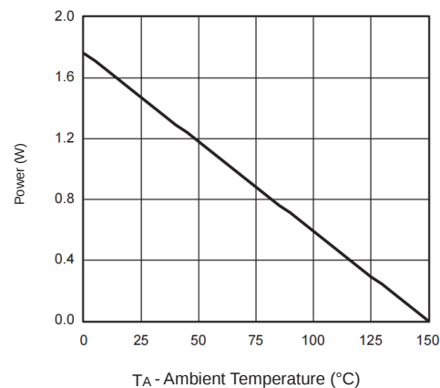
Fig 12. Power, Junction-to-Ambient
