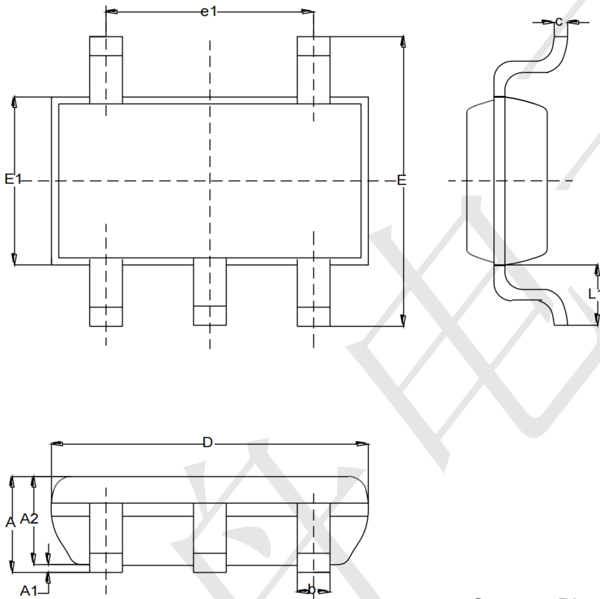
Common Dimensions (Unit of Measure=millimeters)
