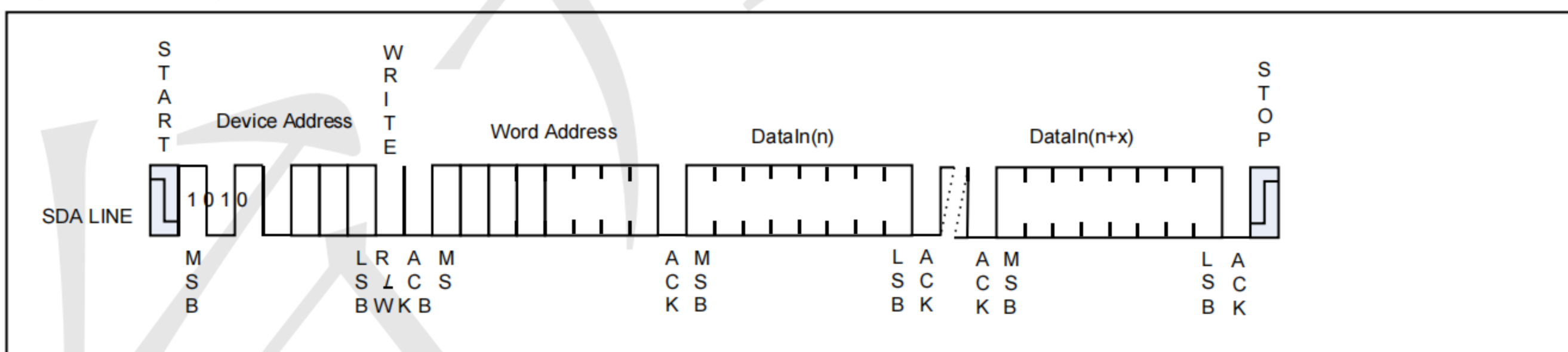
Figure 5-2 Page Write
