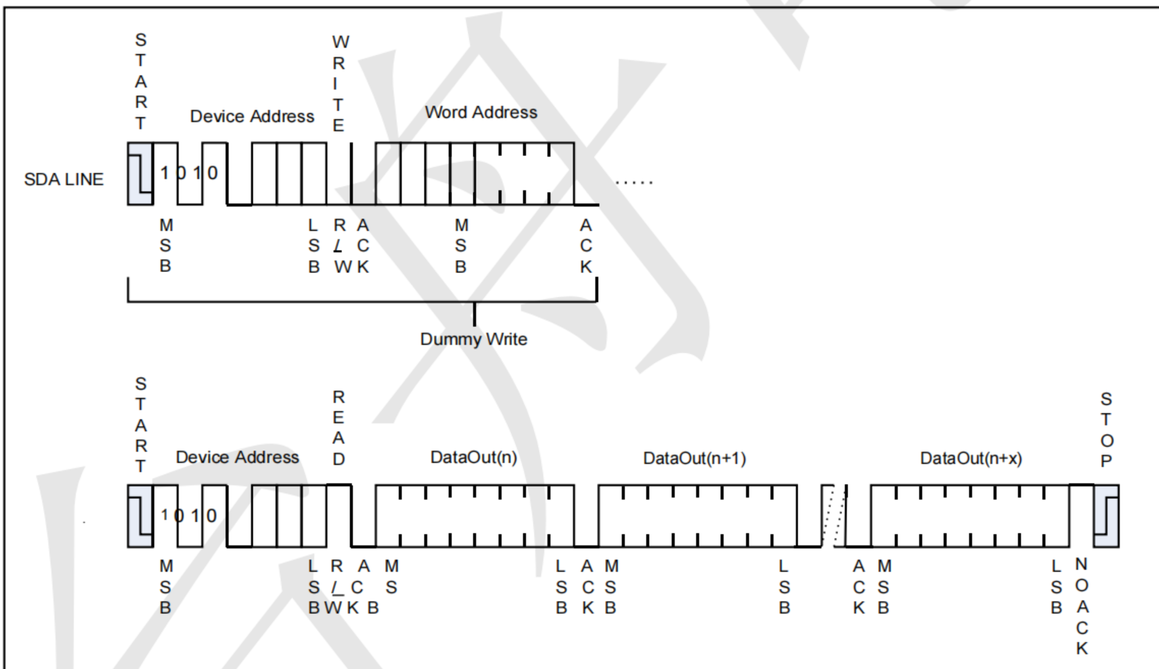
Figure 5-5 Sequential Read
