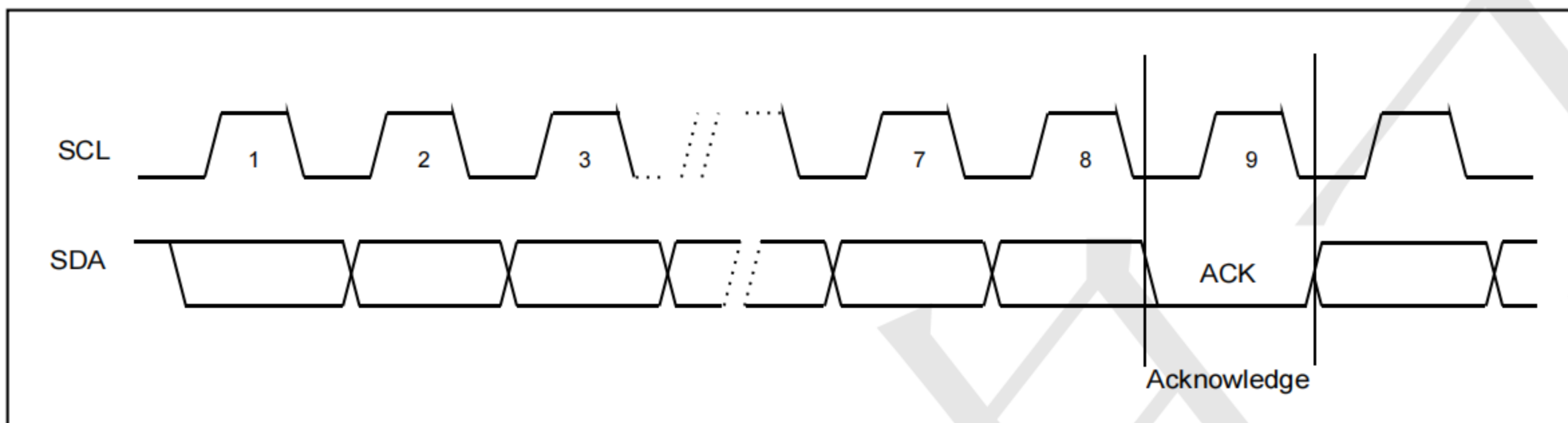
Figure 4-3 Output Acknowledge
