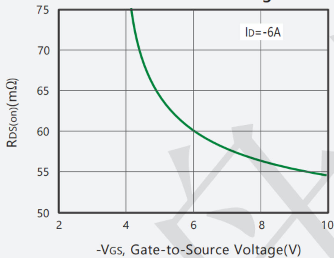
Figure 3. On-Resistance vs. Gate-Source Voltage
