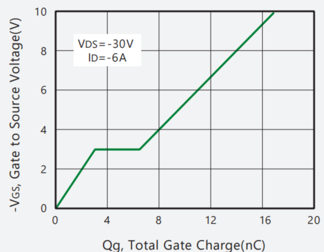
Figure 6. Gate Charge
