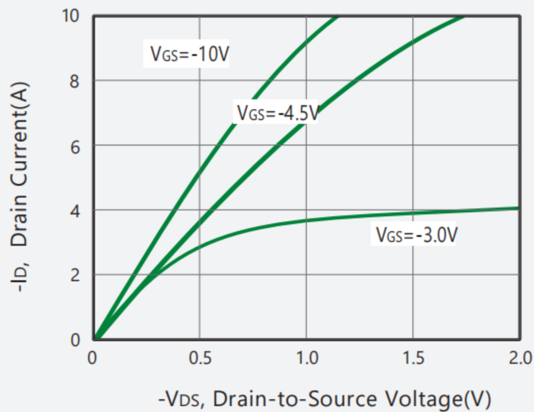
Figure 1. Output Characteristics
