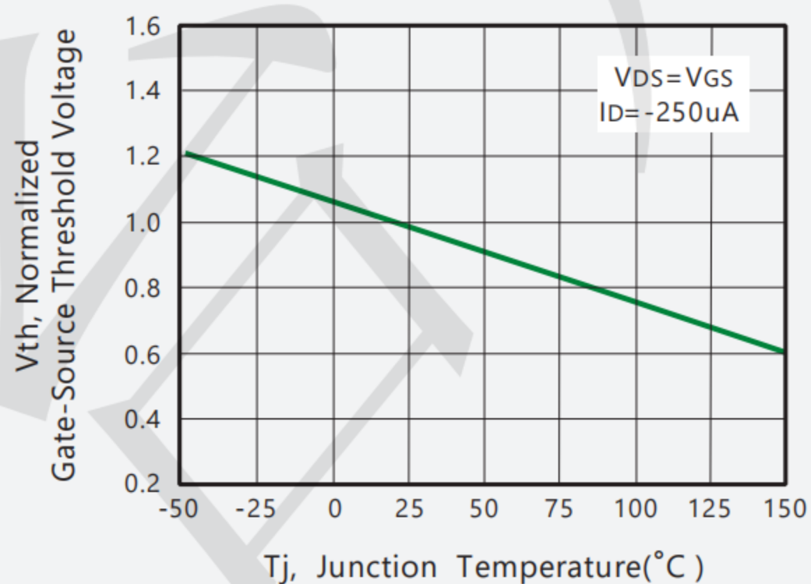
Figure 5. Gate Threshold Variation with Temperature
