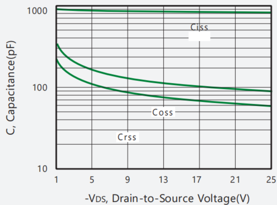
Figure 7. Capacitance
