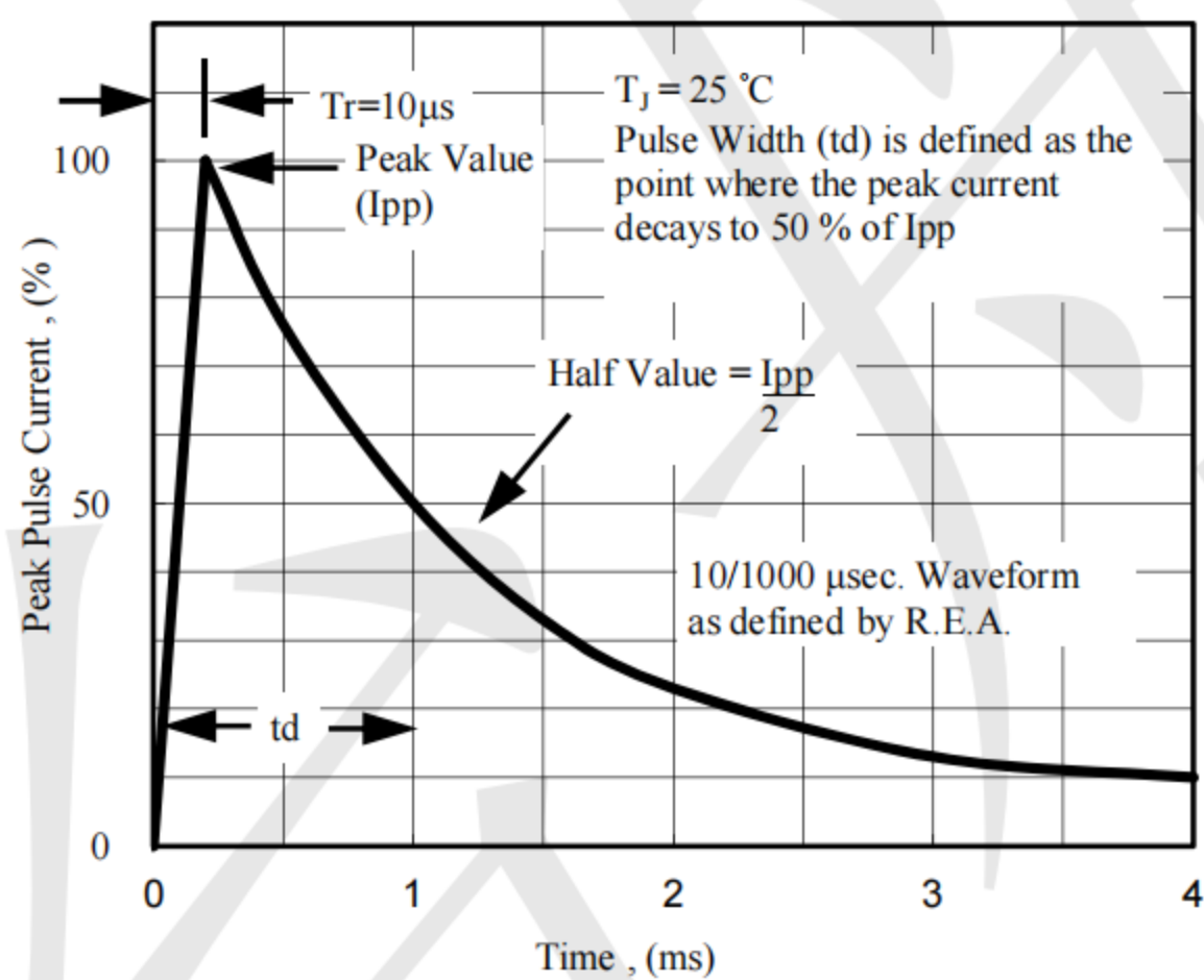
Fig. 5 - Pulse Waveform
