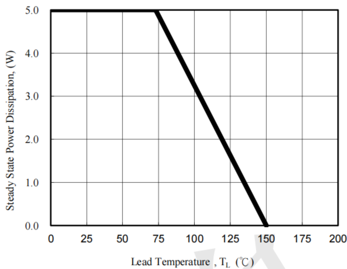
Fig. 3 - Steady State Power Derating Curve
