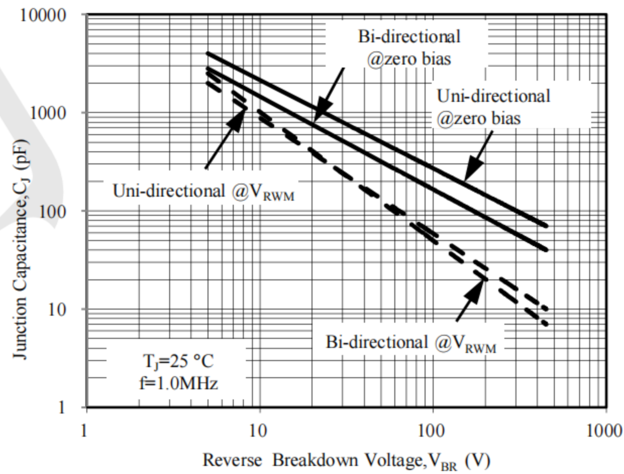
Fig. 6 - Typical Junction Capacitance
