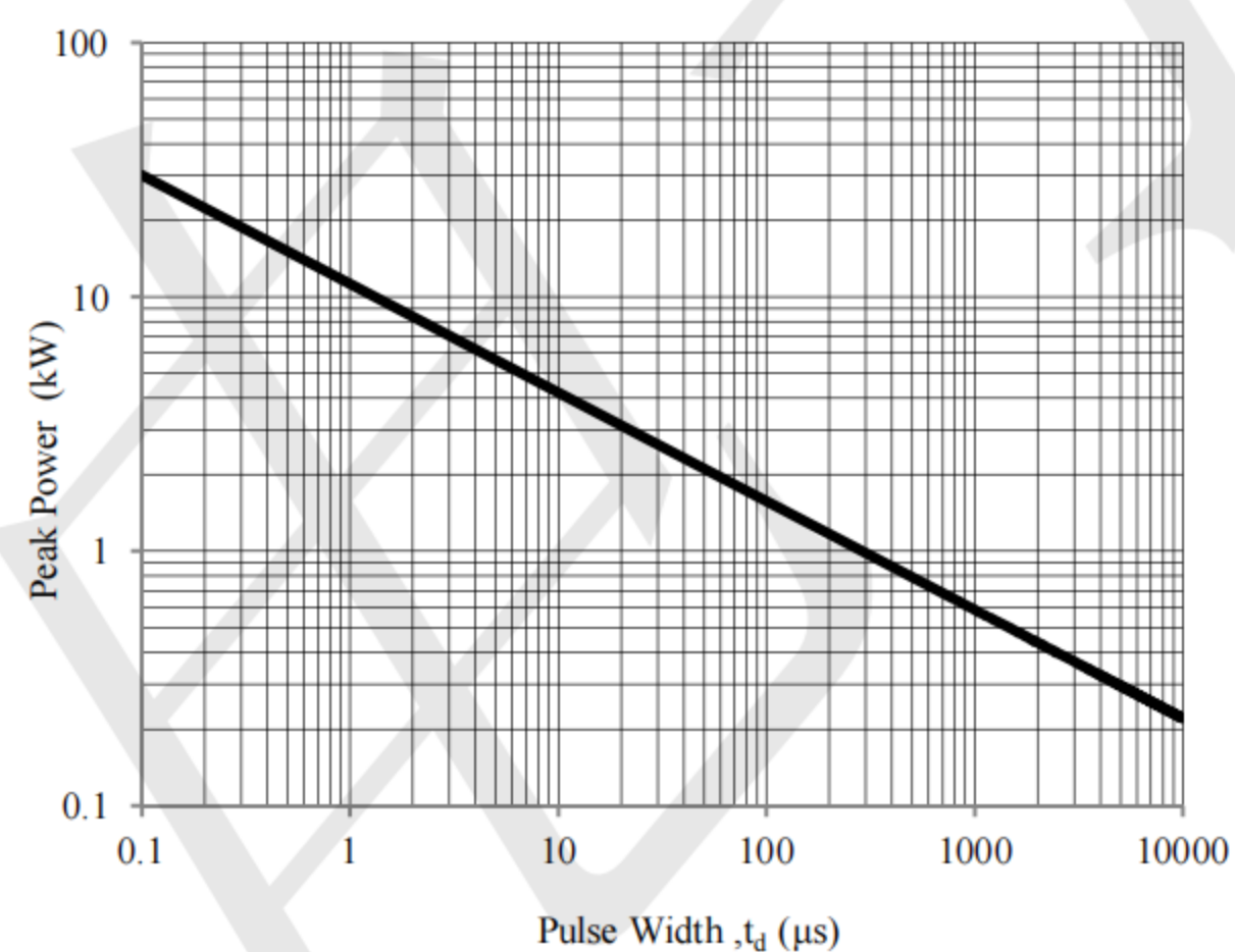
Fig. 4 - Peak Pulse Power Rating Curve
