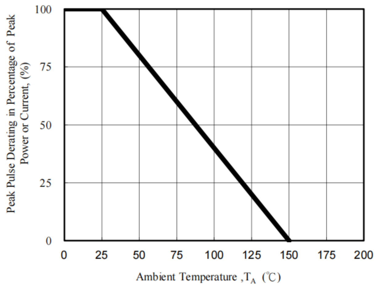
Fig. 1 - Pulse Derating Curve
