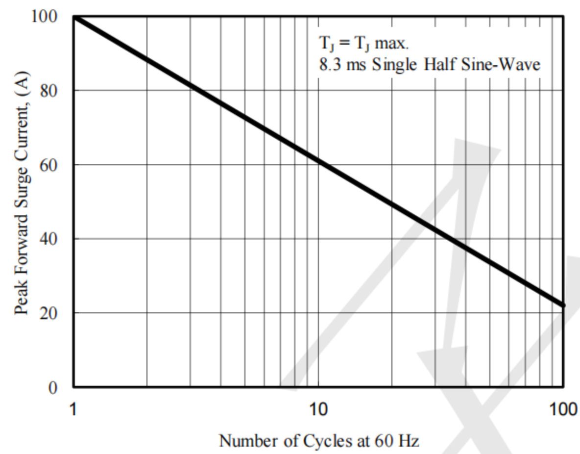
Fig. 2 - Maximum Non-Repetitive Surge Current
