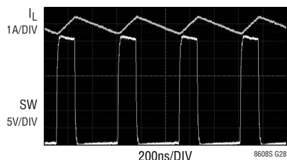
12V IN TO 3.3V OUT AT 1A 2MHz
