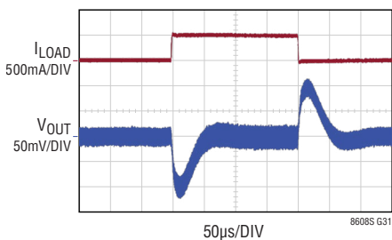
V IN = 12V 0.5A TO 1A C OUT = 47μF f SW = 2MHz
