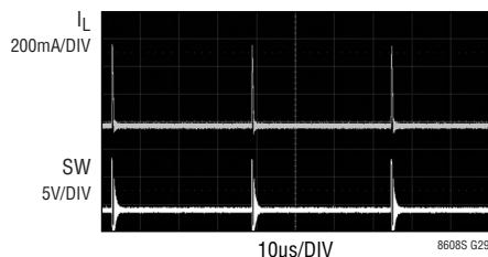
12V IN TO 5V OUT AT 3mA
