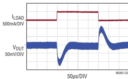
V IN = 24V 0.5A TO 1A C OUT = 47μF f SW = 2MHz
