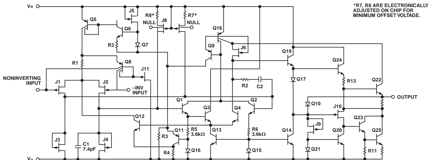
Figure 1. Simplified Schematic
