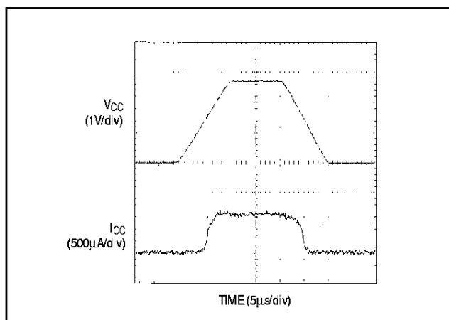
Figure 12. Power-Up Supply Current
