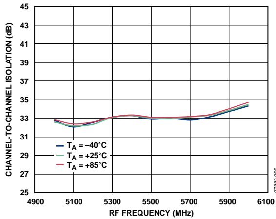
Figure 66. Channel-to-Channel Isolation
