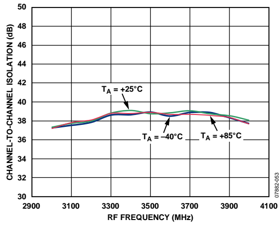
Figure 53. Channel-to-Channel Isolation
