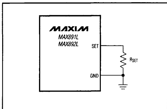
Figure 2. Setting the Current Limit
