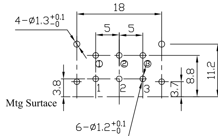
Mounting hole detail
