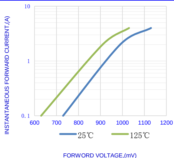
Fig.2-TYPICAL INSTANTANEOUS FORWARD
