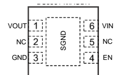
DFN2x2-6L
