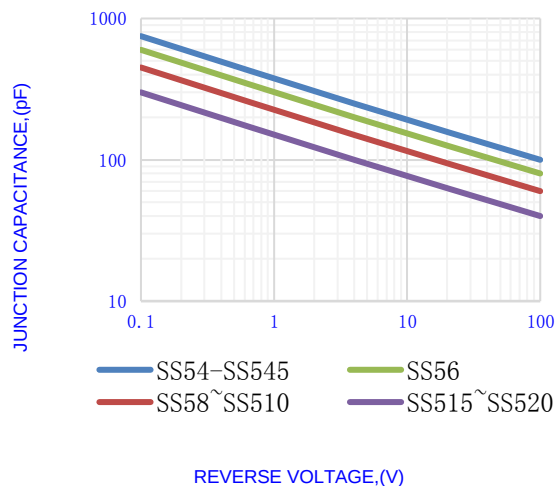
Fig.4-TYPICAL JUNCTION CAPACITANCE
