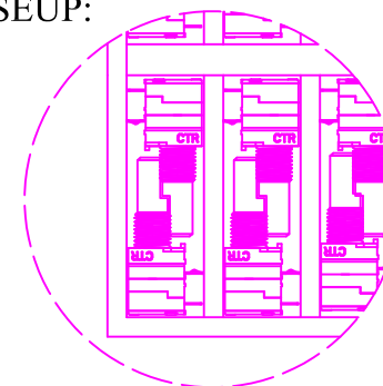
A部局部视图 "A" CLOSEUP:
