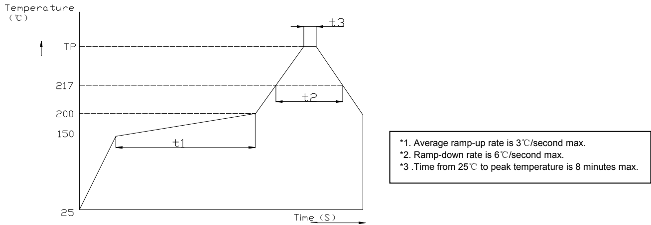
Allowable Range of Peak Temperature
