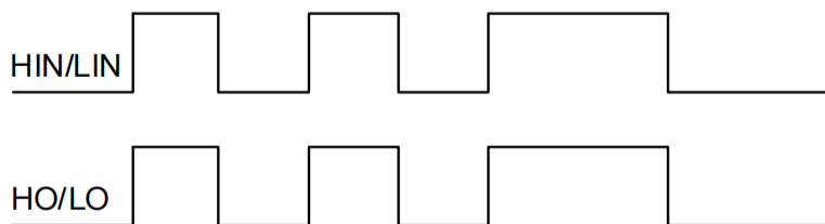
Figure 5. UCC27710 Input and output timing waveform
