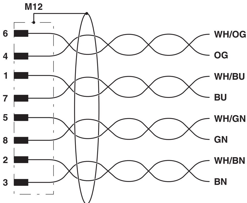
Circuit diagram
