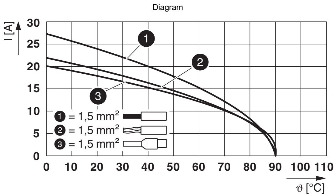
Derating diagram for 1.5 mm²
