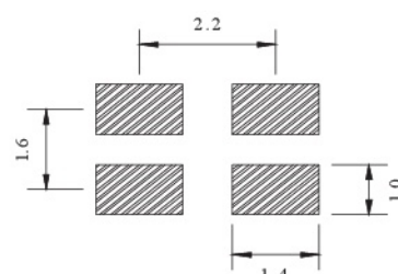
<SUGGESTED LAYOUT>
