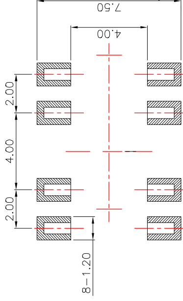
P. C. B MOUNTING PATTERN DIMENSION the following soldering are recommended for reflow soldering
