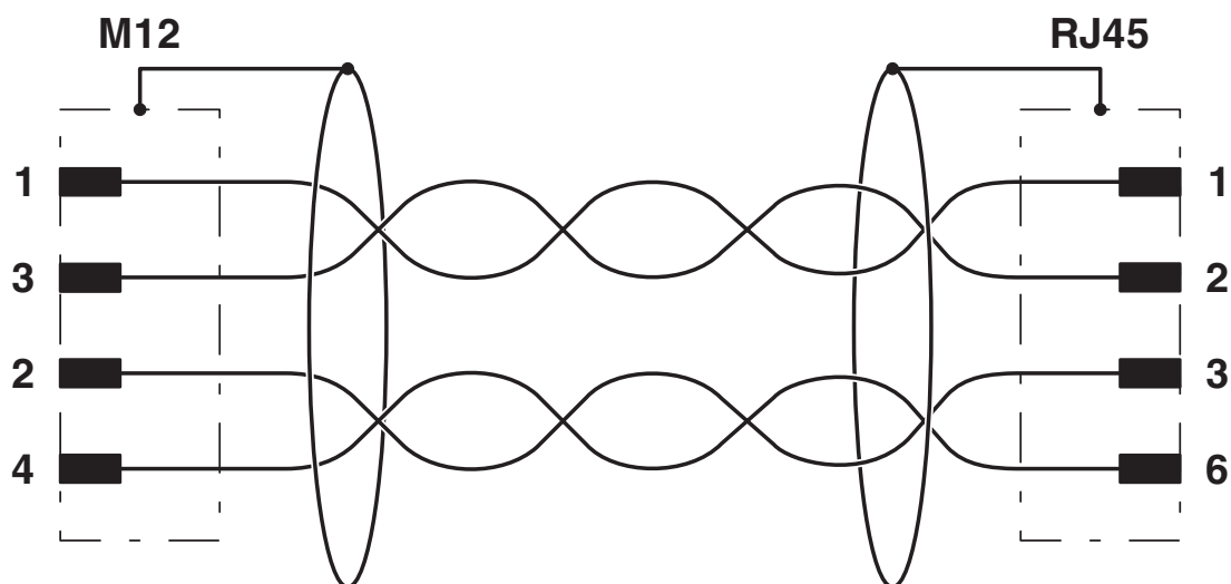
Circuit diagram
