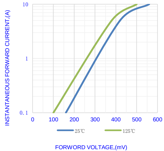
Fig.2-TYPICAL INSTANTANEOUS FORWARD
