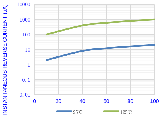
Fig.3-TYPICAL REVERSE CHARACTERISTICS
