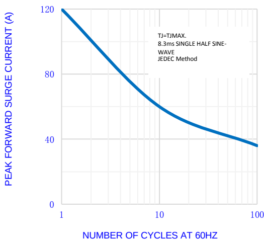
Fig.5-MAX. NON-REPETITIVE SURGE CURRENT
