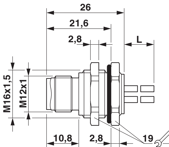
Dimensional drawing
