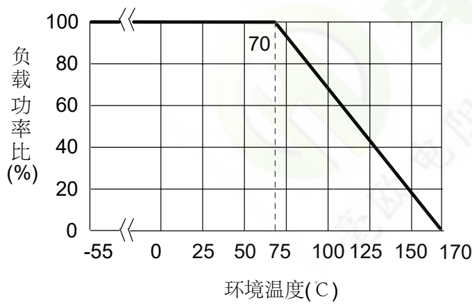
功率曲线 Power Curve
