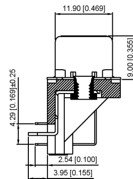
TYPE 1: riveting(铆合) Profile B-B
