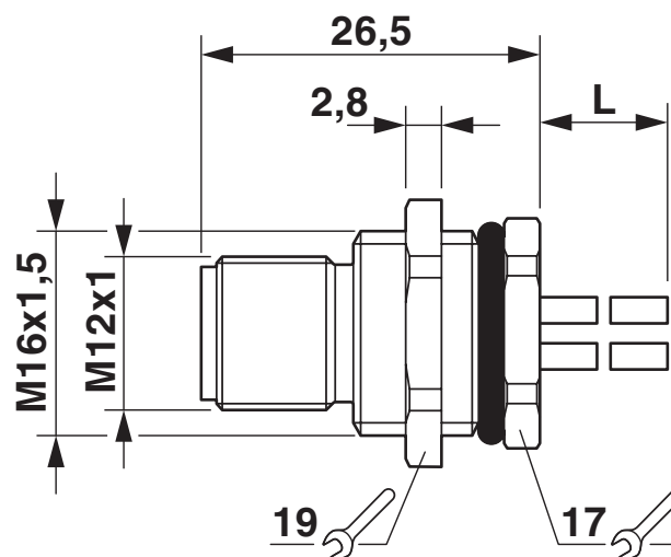
Dimensional drawing
