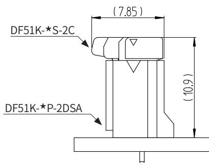
[Single-row]
