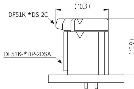
[Double-row]
