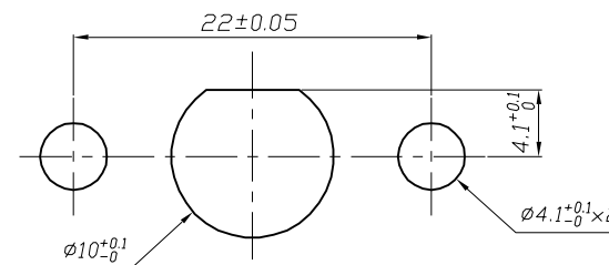
PANEL CUTOUT
