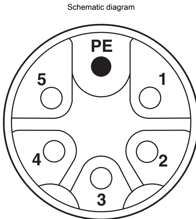
Pin assignment of M12 socket, 6-pos., M-coded, socket side view
