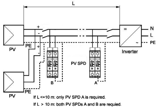
Fig 2: Positions of SPDs (T configuration) in the DC part stipulated in Guide IEC 61643-32
