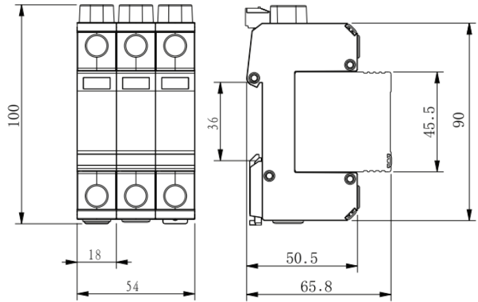
3) Three poles, "Y" configuration
