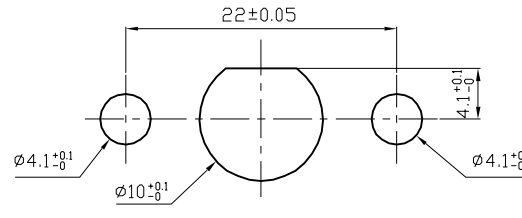
PANEL CUTOUT
