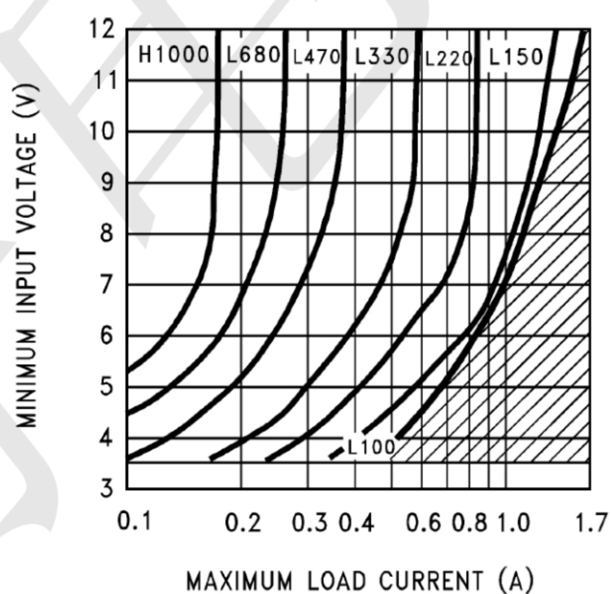
FIGURE 8. LM2577S-ADJ-15
