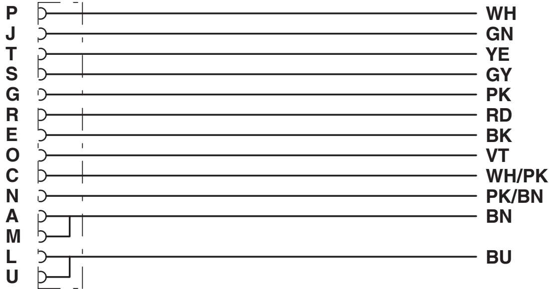
Circuit diagram
