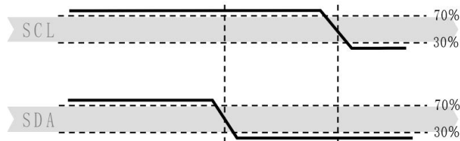
Figure 18. Start transmission status (S)
