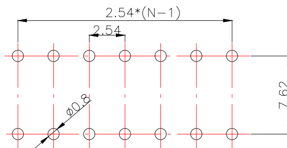
[P.C.B.LAYOUT]
