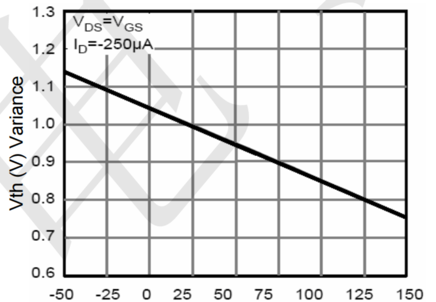
Figure 10 V_{GS(th)} vs Junction Temperature
