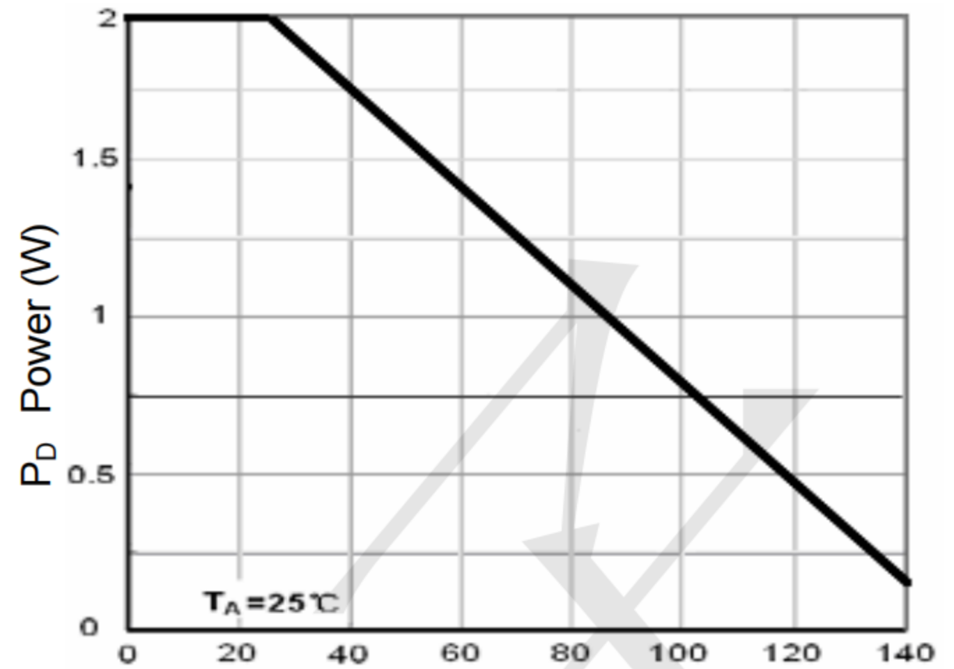
Figure 9 Power Dissipation
