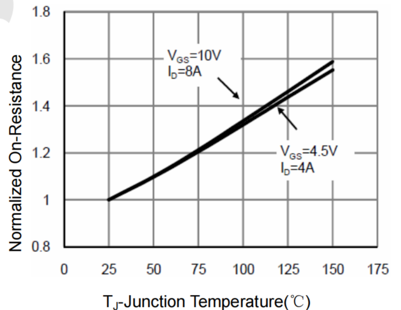
Figure 6 Drain-Source On-Resistance
