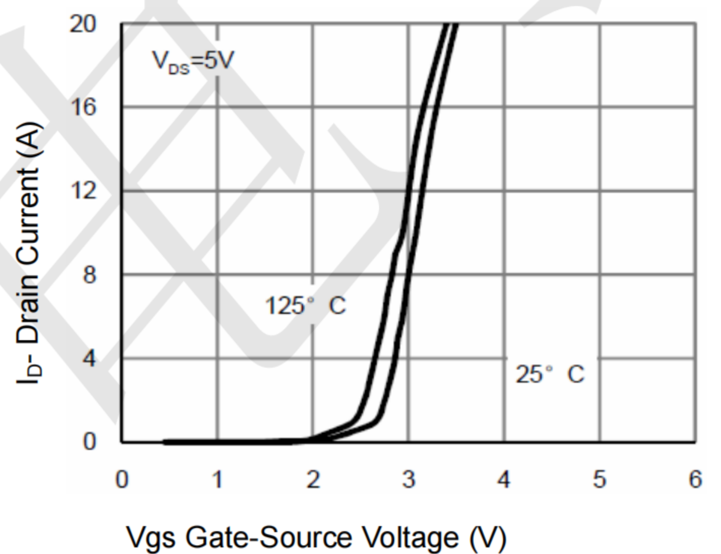
Figure 4 Transfer Characteristics
