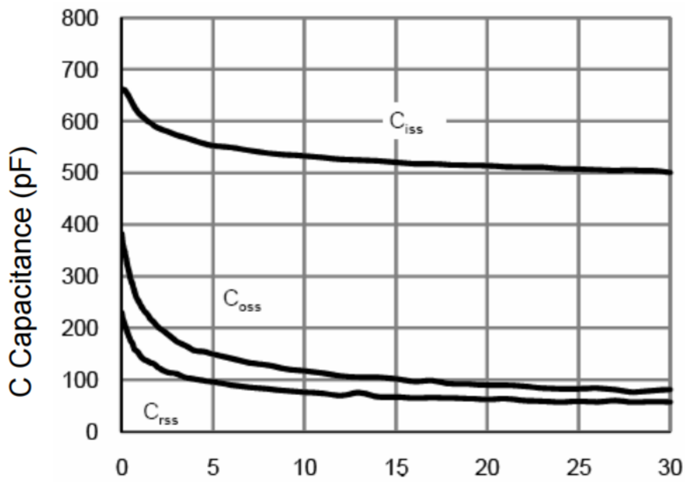
Figure 7 Capacitance vs Vds
