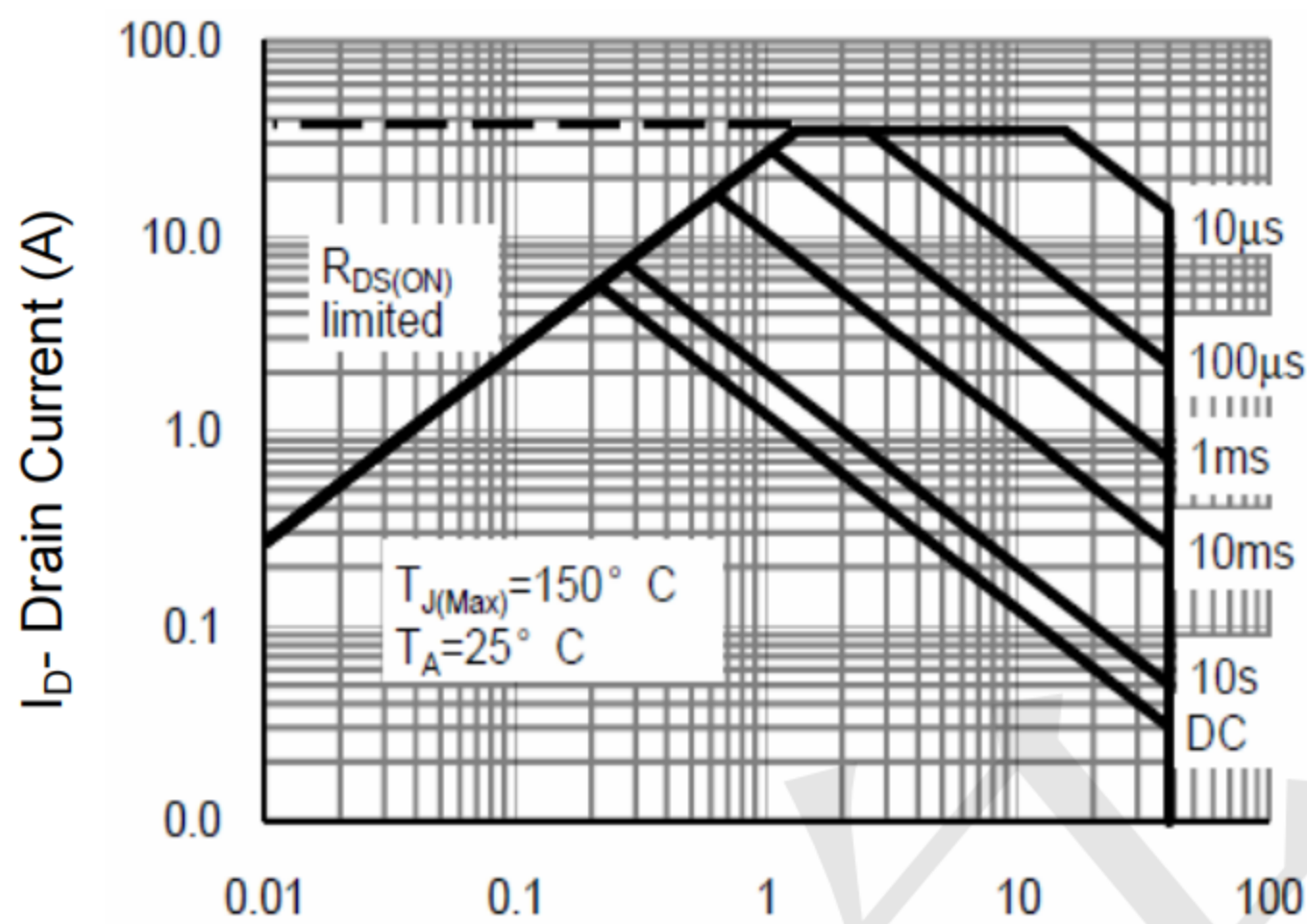
Figure 8 Safe Operation Area
