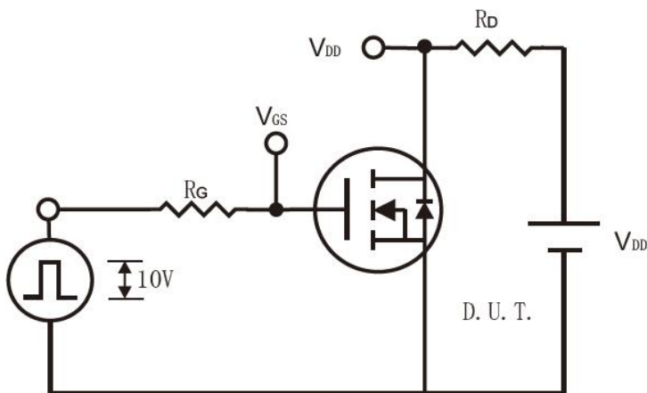
Switching Test Circuit
