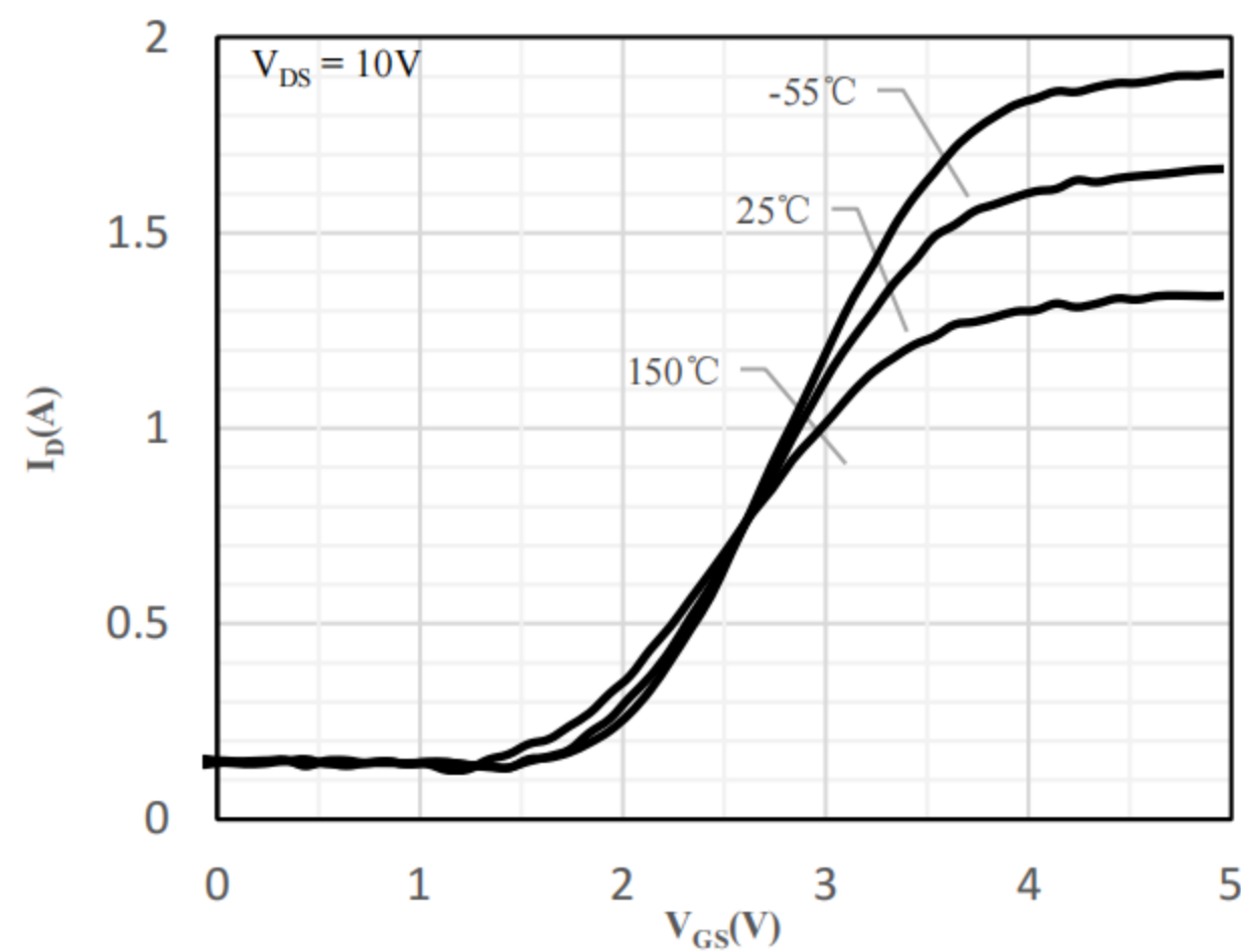
Fig 6 Transfer Characteristics
