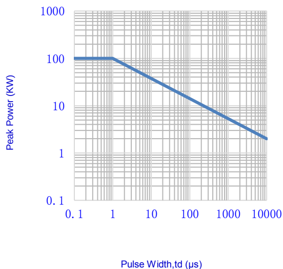
Fig.3- Peak Pulse Power Rating Curve
