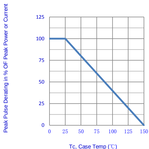
Fig.1-Pulse Derating Curve
