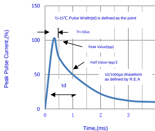
Fig.6-Pulse Waveform
