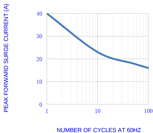
Fig.5-MAX. NON-REPETITIVE SURGE CURRENT
