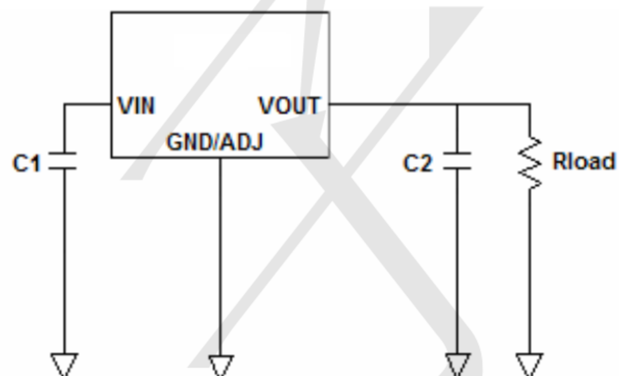
TP1117 fixed output
