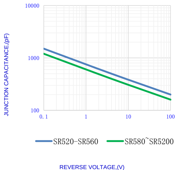
Fig.4-TYPICAL JUNCTION CAPACITANCE
