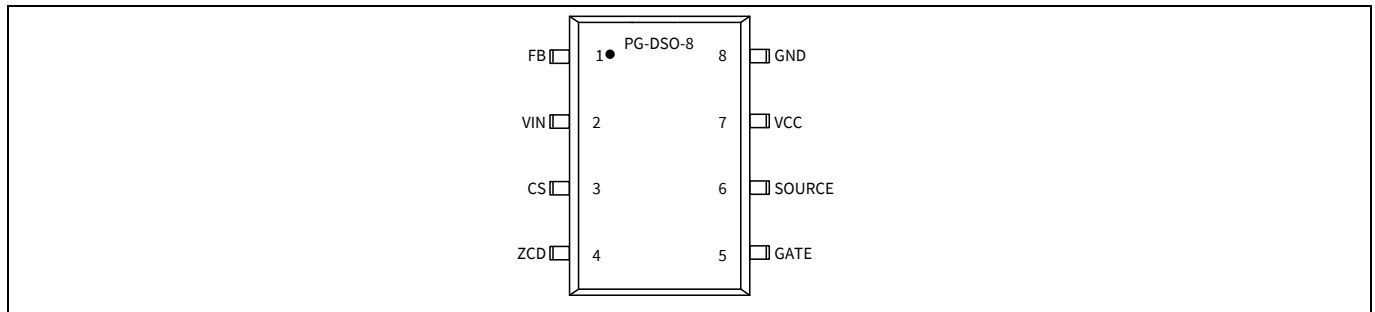
Figure 2 Pin Configuration
